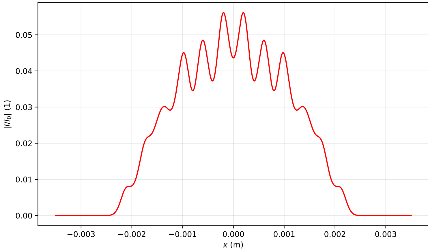
Intensity profile I(x, y = 0, z = 3.821)/I_0 , P_{in}=5.5P_{cr} , artificial time
